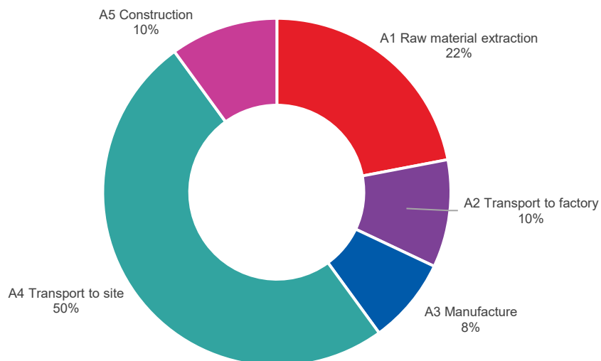
Figure 2 CLT approximate percentage of A1-A5 carbon each stage accounts for, based on multiple resources including EPDs and various data extracts. Data is based on European manufacture and transport from Austria to the UK.
