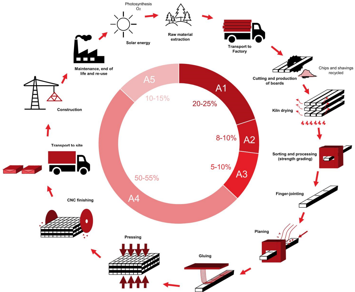
Figure 11 Typical supply chain process for CLT & Glulam products [15].
